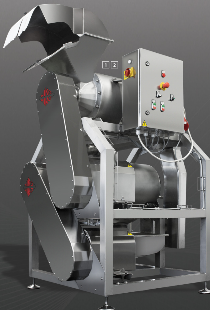
STONE FRUIT PROCESSING LINE (option 2)
